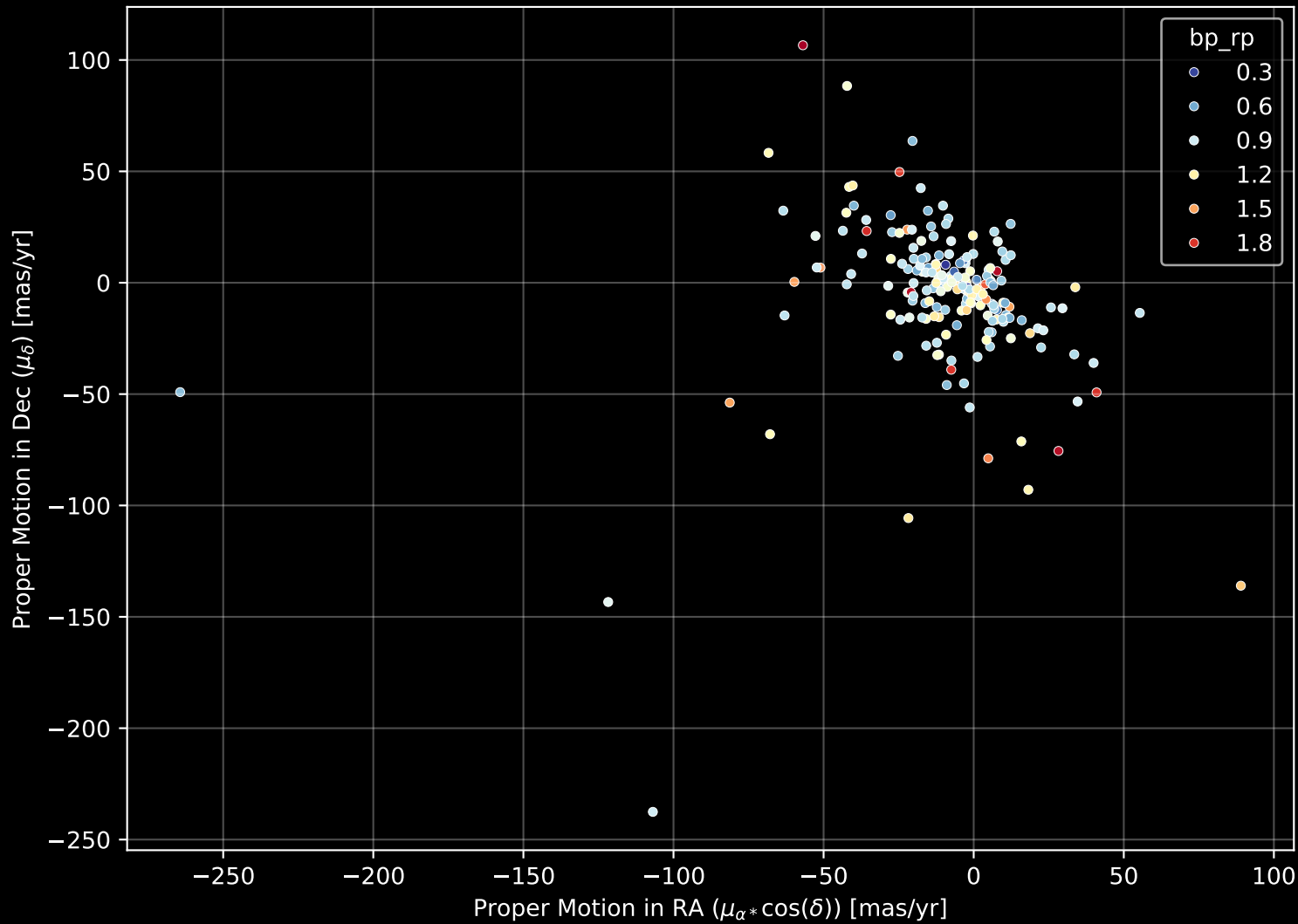
APOGEE DR17 Field: [076+50_MGA] Proper Motion Diagram (n= 202)
