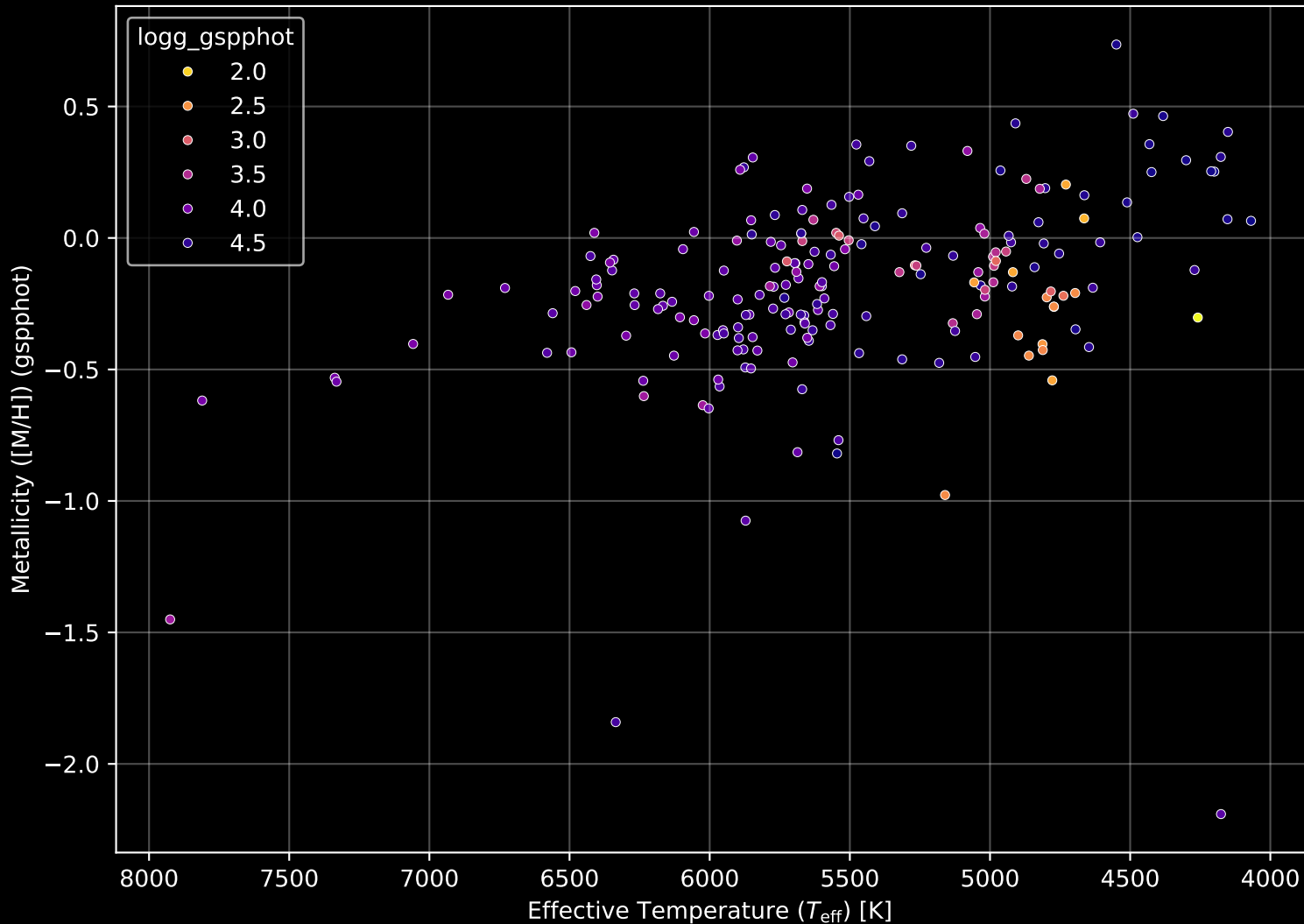
APOGEE DR17 Field: [076+50_MGA] Stellar Population Parameters (n= 202)
