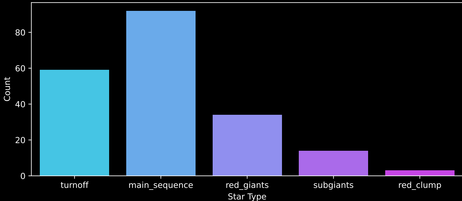
APOGEE DR17 Field: [076+50_MGA] Count plot of Star Type
