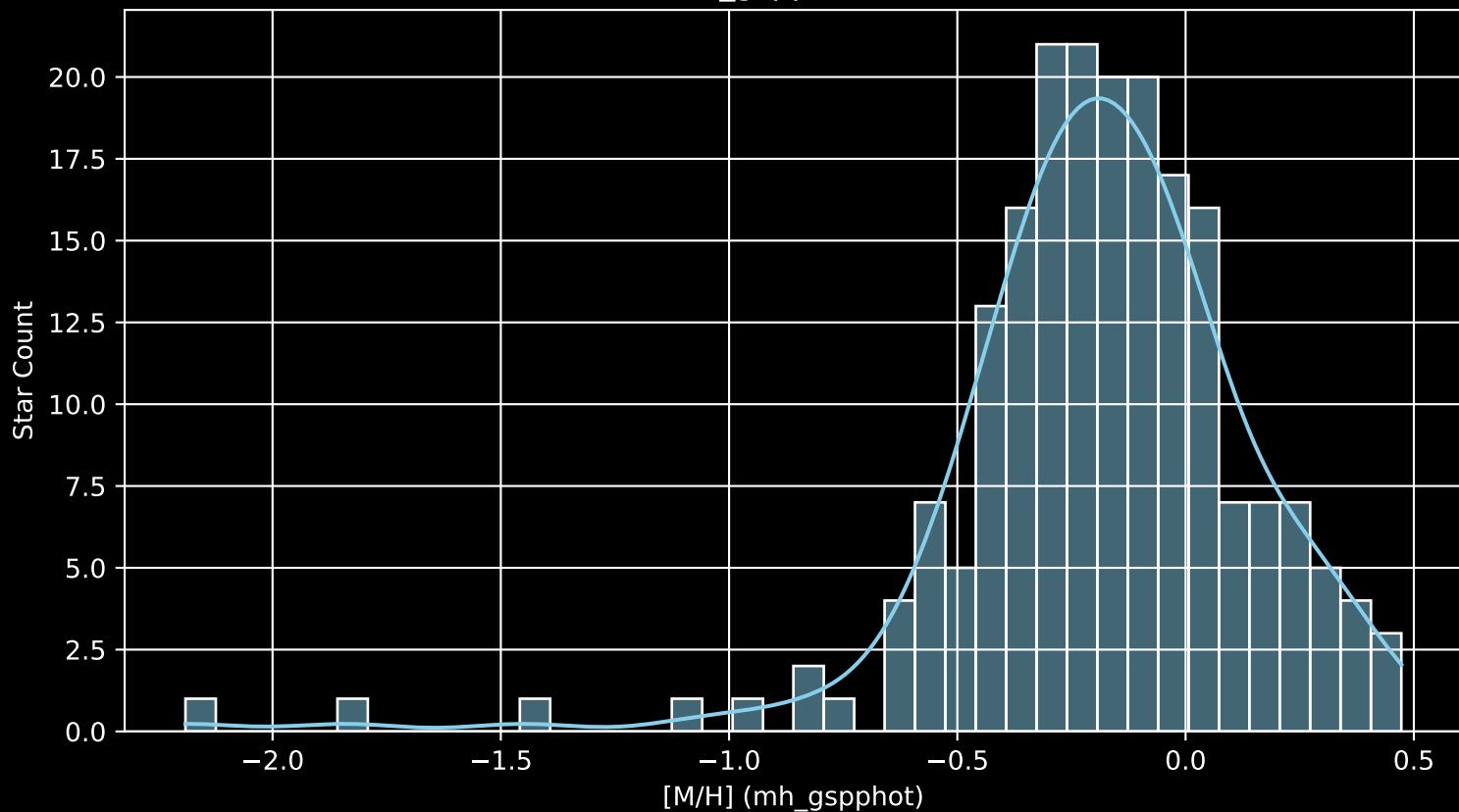
APOGEE DR17 Field: [076+50_MGA [M/H] (mh_gspphot) (n= 201)
