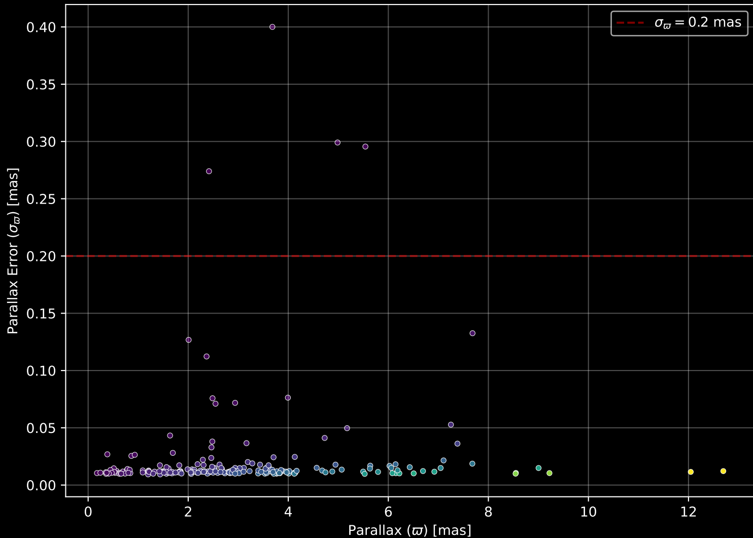
APOGEE DR17 Field: [076+50_MGA] Parallax Quality (n= 202)
