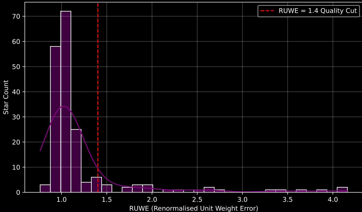
GAPOGEE DR17 Field [076+50_MGA] RUWE Distribution (n= 191)
